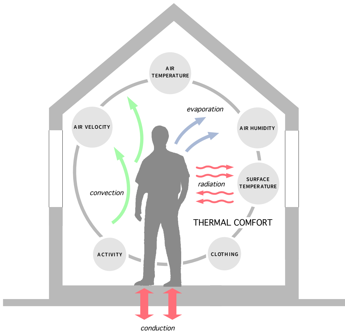
Figure 2: Factors affecting thermal comfort.
