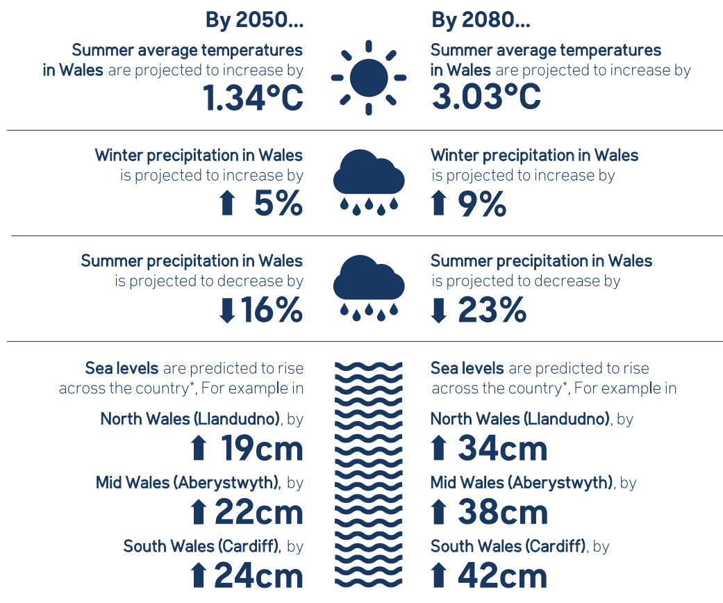
Figure 5: Climate Change predictions by 2050 and 2080 taken from the UK Climate Projections (UKCP18) dataset. 3
