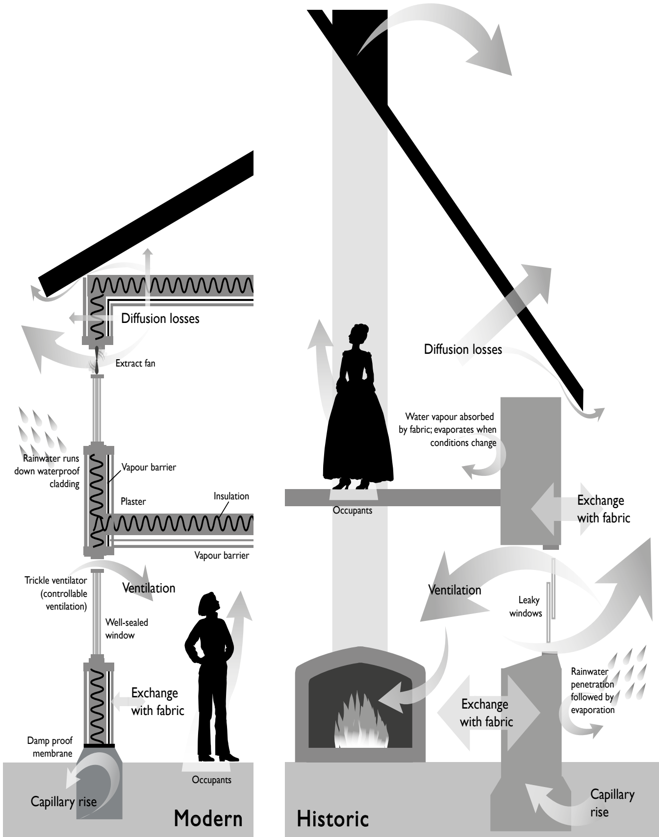
Figure 4: Typical differences in the movement of moisture and air in modern and traditional construction.
