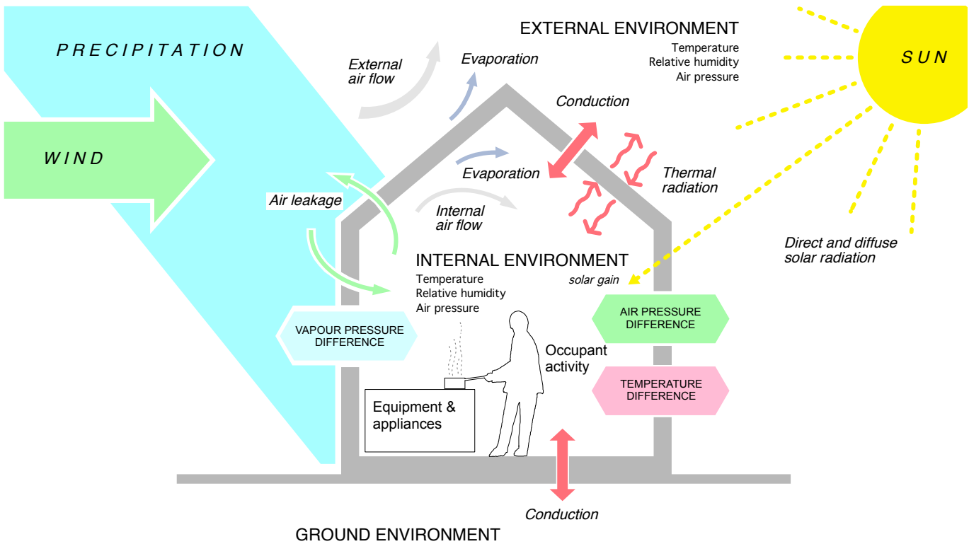
Figure 7: Interactions between the building envelope and the environment.
